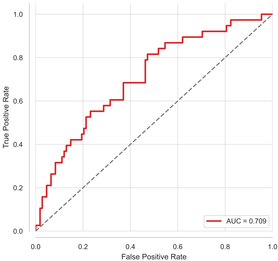
ROC Curve - LR
